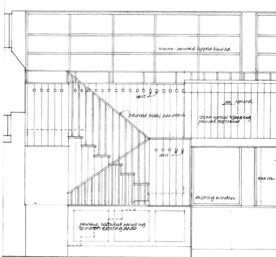
ELEVATION 1-20
